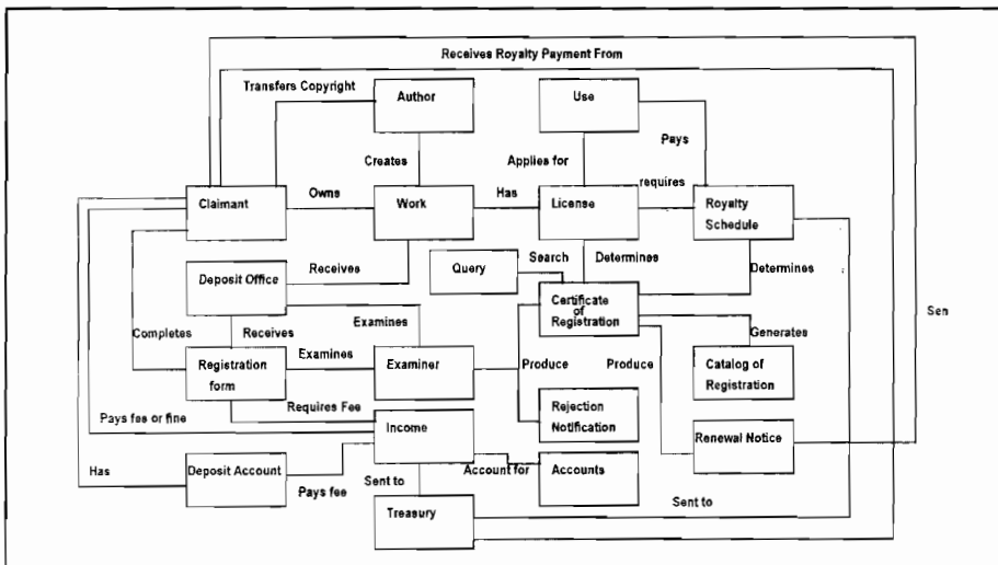
Figure 2 A High Level Object Model for he Deposit and Copyright Process
