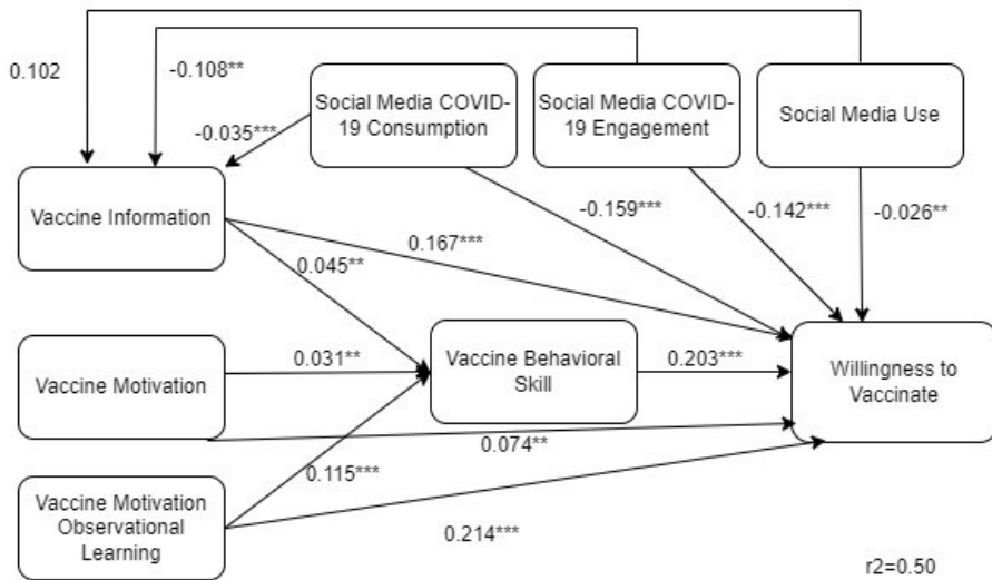
Figure 2: SEM Coefficients are Standardized Path Coefficients
